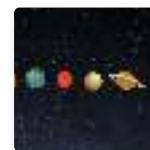
Solar system
